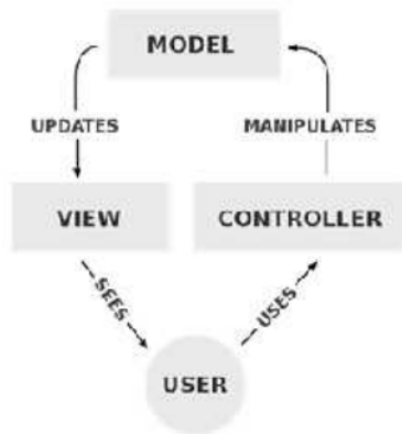
Gambar 1. Model-View-Controller
