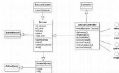
Gambar 4. Class Diagram Jurusan
