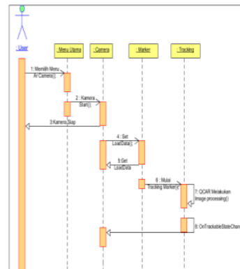
Gambar 6. Sequence Diagram
