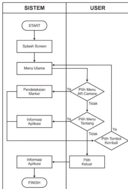
Gambar 3. Flowchart
