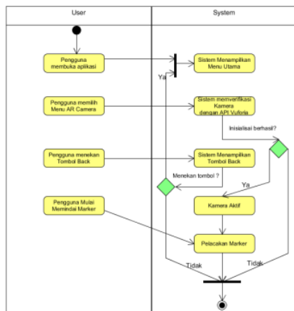
Gambar 4. Activity Diagram
