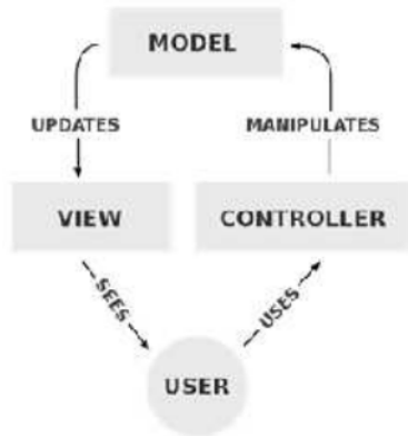
Gambar 1. Model-View-Controller
